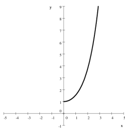
restricted \cosh x
