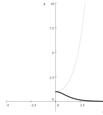
\operatorname{sech} x restricted
