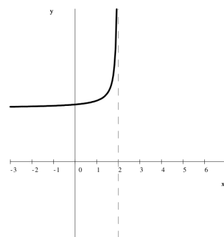
Vertical asymptote at x = 2
