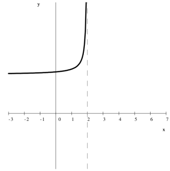
Vertical asymptote at x = 2
